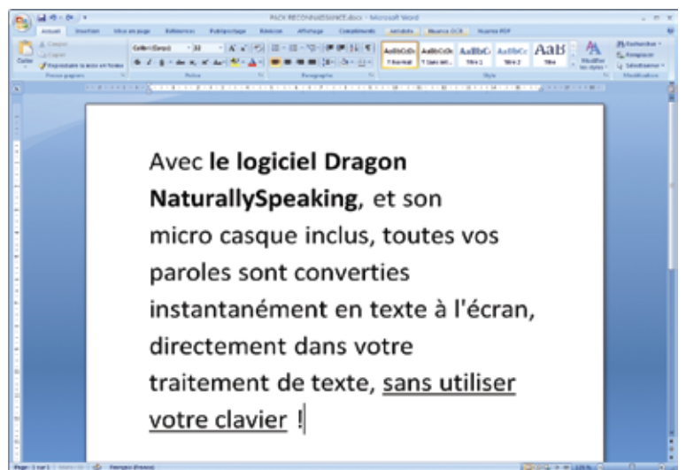
Dragon NaturallySpeaking
