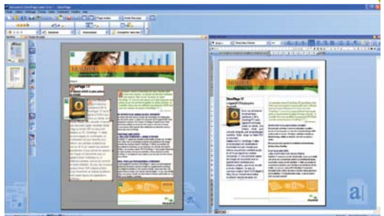
OmniPage
